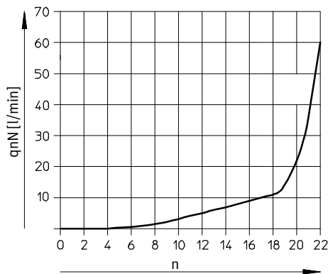
Standard nominal flow rate q_{nN} at p > 5 bar as a function of turns of the adjusting screw n
