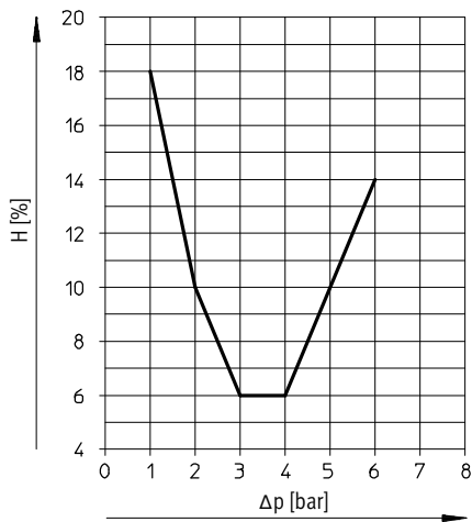
Hysteresis H as a function of the differential pressure Δp
