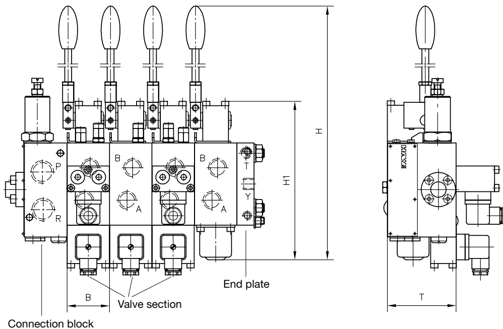
Connection block
