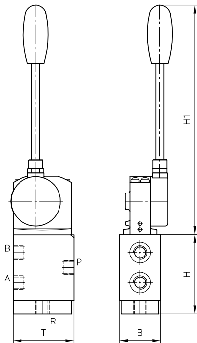
SG with manual actuation
