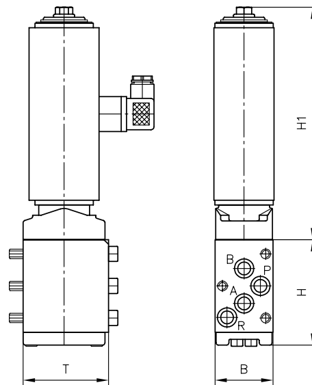
SP with solenoid actuation
