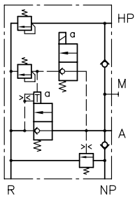
CR 4M; CR 5M
