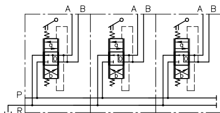
Valve bank
