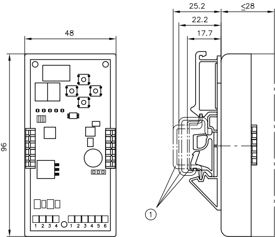
1 Standard support rails
