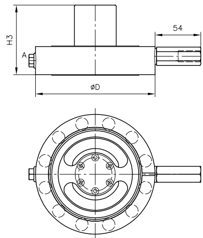
Pre-fill valve
