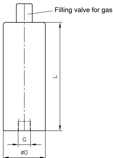
1 Gas-filling valve
