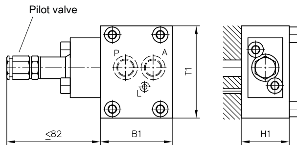
1 Pilot valve
