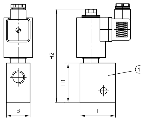
1 Connection block
